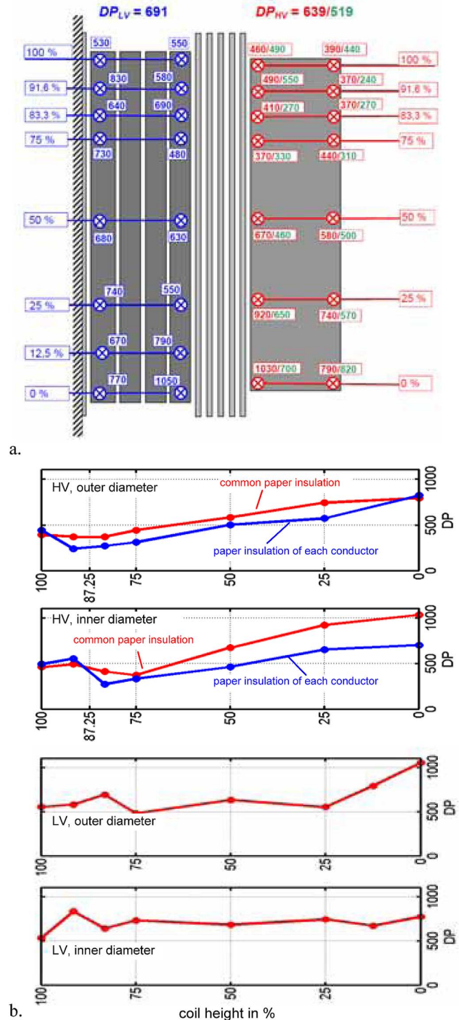
Fig. 4. DP of paper samples taken from transformer M5 according to Fig. 3: (a) DP values of individual paper samples, green DP figures: paper insulation of the individual conductors, red DP figures: common paper insulation of a twin conductor. (b) DP profile along the HV and LV coil.
