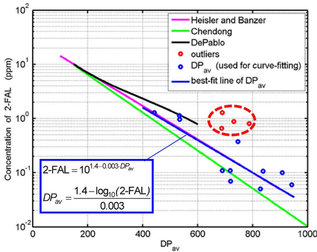
Fig. 7. Correlation between the concentration of 2-FAL in the oil and average DP according to (7) for the grid transformers given in Fig. 3 without using data of transformers N11 to N14.
