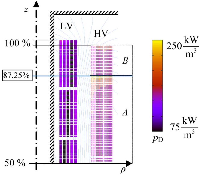
Fig. 5. Distribution winding losses p_D calculated for transformer M5 in Fig. 3.
