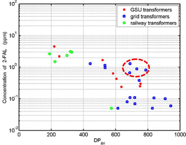
Fig. 3. Entirety of all investigated power transformers sorted into three groups.
