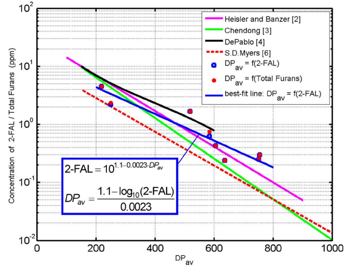
Fig. 6. Correlation between concentration of 2-FAL and total furans in the oil and average DP according to (7) for GSU transformers given in Fig. 3.
